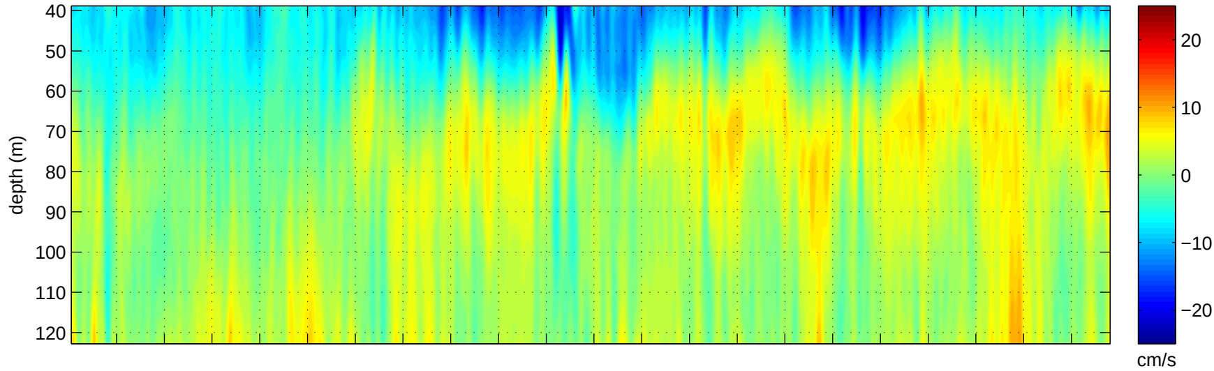
Along Channel (−5.5° True) Current
