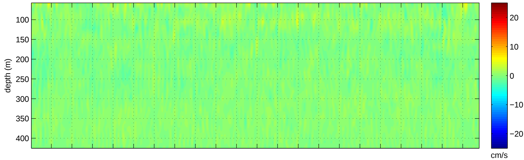
Cross Channel (120° True) Current
