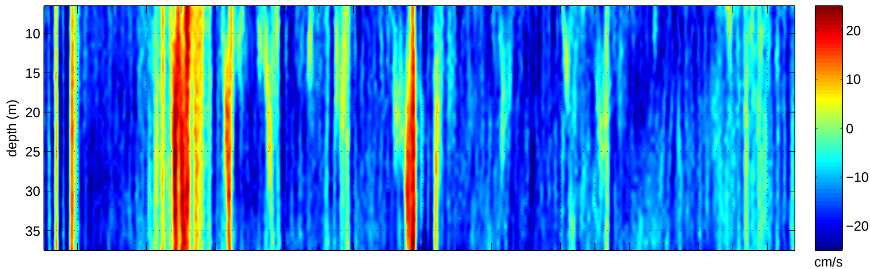
Cross Channel (120° True) Current
