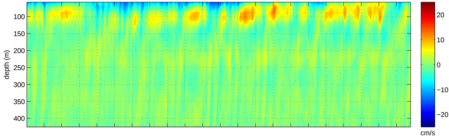
Along Channel (30° True) Current
