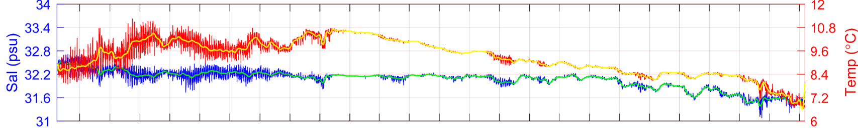
Microcat at 42 m
