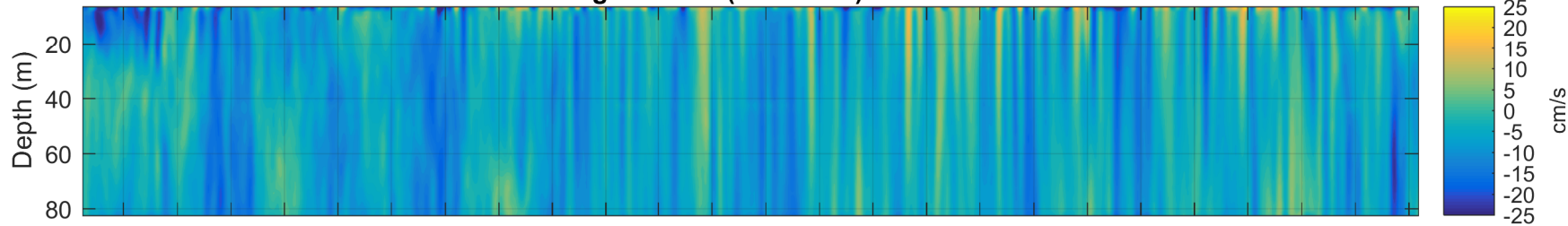
Chat2-1 Along Channel (360° True) Current
