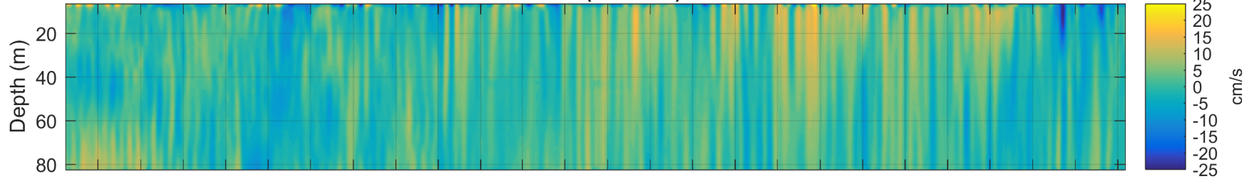
Cross Channel (90° True) Current
