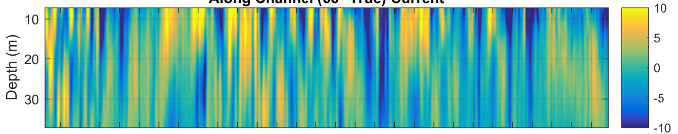
ESP2-A Along Channel (66° True) Current
