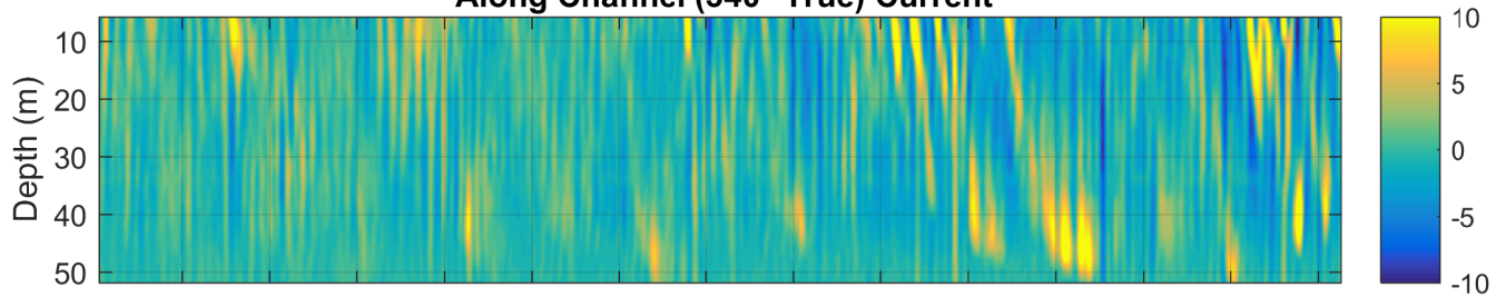
EF04-M Along Channel (340° True) Current
