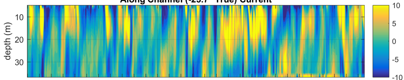
Cook1-A Along Channel (-23.7° True) Current
